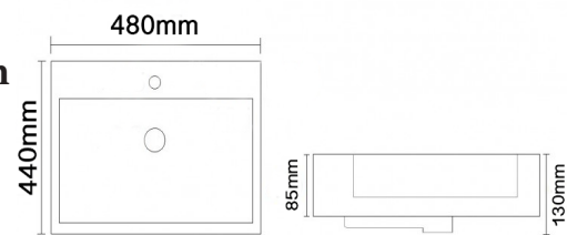
Quantum Series Low Profile Above Counter Basin D-340
